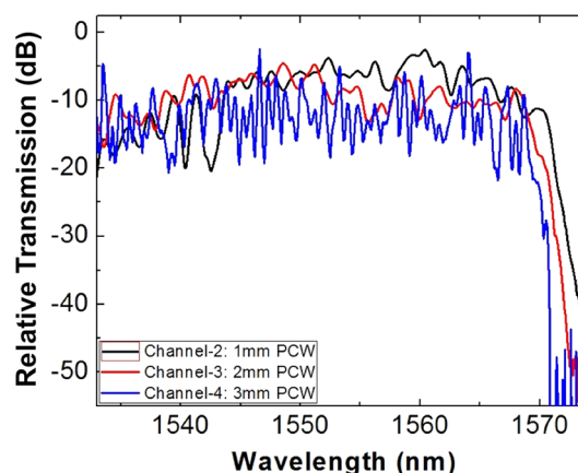
FIG. 2. Transmission spectra of the channels containing 1–3 mm PCWs.
